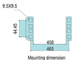
Mounting dimension
